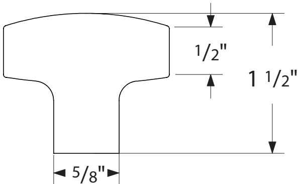
Mod Hex Knob 1-1/2" 86458
