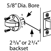
Thumbturn Privacy Inside Trim
