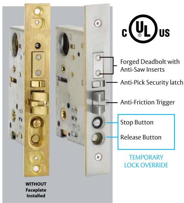
F20 Mortise Lock Box
