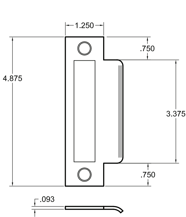
Brass Standard Strike Plate
