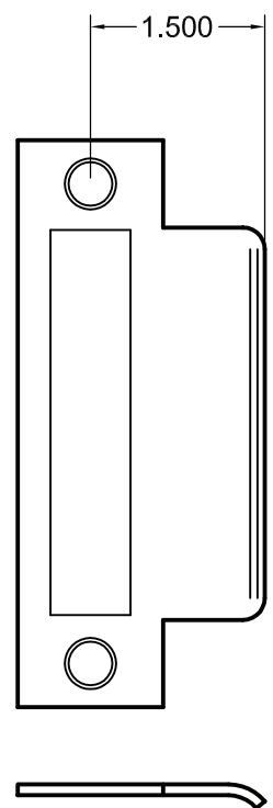
Brass Extended Strike Plate
